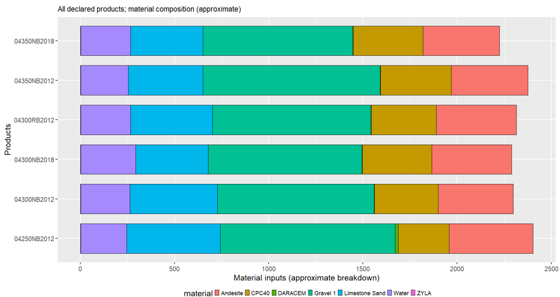
Figure 1: Approximate material composition - All declared products per 1 m3 of concrete. Note: presented breakdown is approximate to ensure confidentiality.
